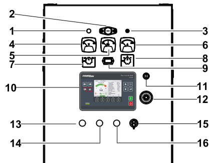
Control cabinet
