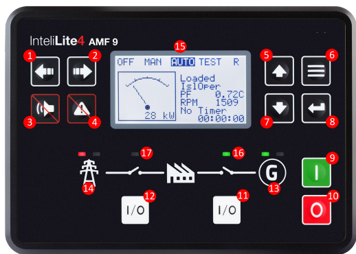
Control module
